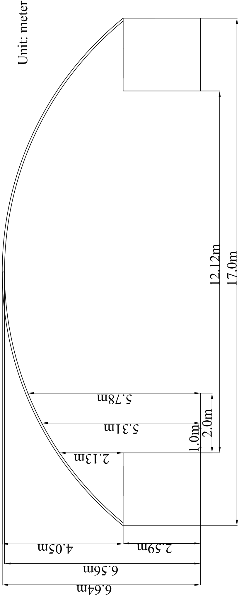
W12.12(17) x L12.19 x H4.05m Over Container Shelter 12/17
