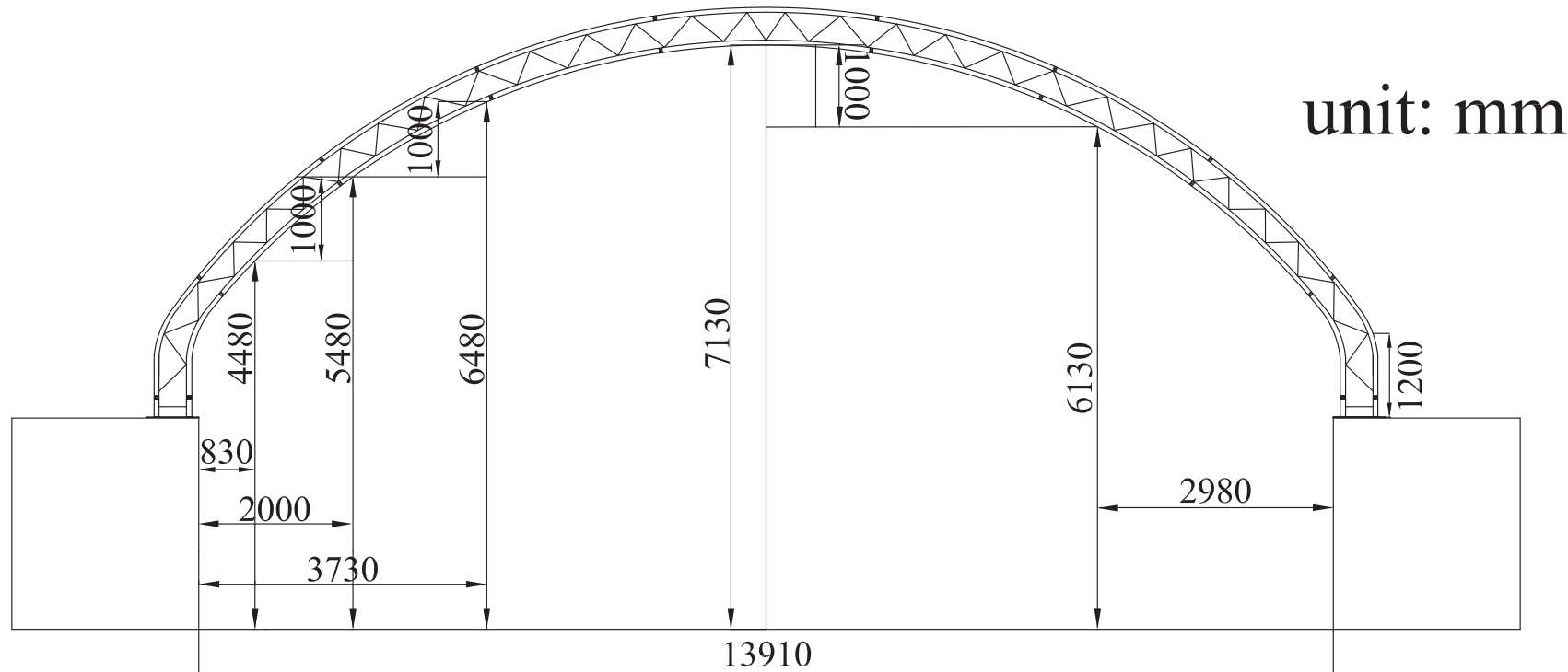
14m wide container shelter
